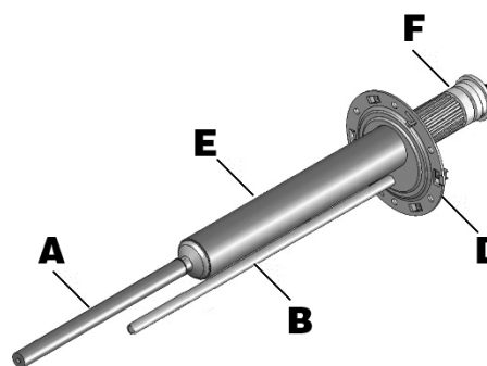
Picture 2- Steatite heating element + magnesium anode
