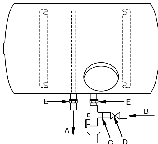
Picture 10 - Horizontal model on ring nut
