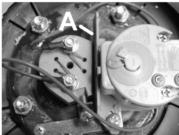
Picture 17 - Plastic separator / A: plastic separator
