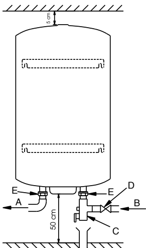
Picture 6 - Installation values
