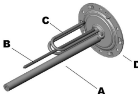
Picture 1- Immersion heating element + magnesium anode
