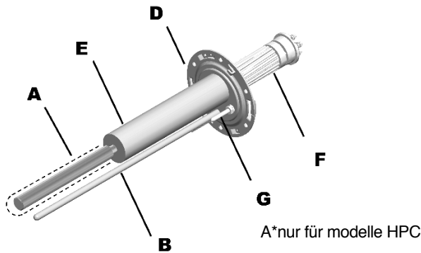
Abbildung 3 - Steatit-Heizwiderstand + PROfessional TECHanode
